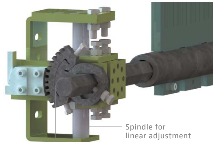
Adapter 830 for torsion adjustment
