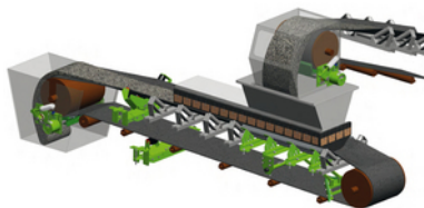
Complete conveyor system with elements from the STARCLEAN® modular system series
